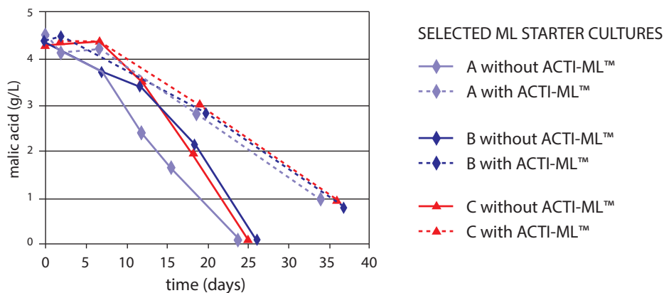
Kinetics of malic acid degradation in a Chardonnay wine (alcohol 14,1% vol, T-SO 2 14, ppm pH 3,3) after direct inoculation with selected ML starter cultures with and without addition of ACTI-ML™.
