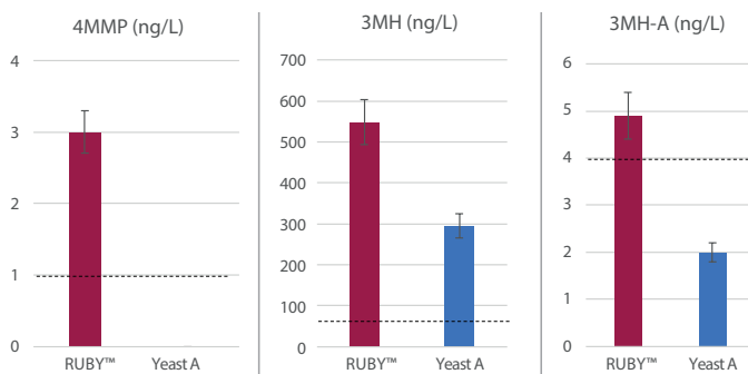
Thiols analysis in bottled wines. Trial in Tempranillo, Spain (14.5% v/v; pH=3.8; Total Acidity=5.2 g/L TH 2 )
